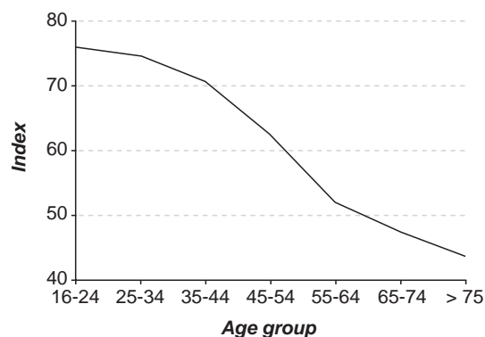
Figure 2. Plot of health status index (first dimension of correspondence analysis) against age group.
