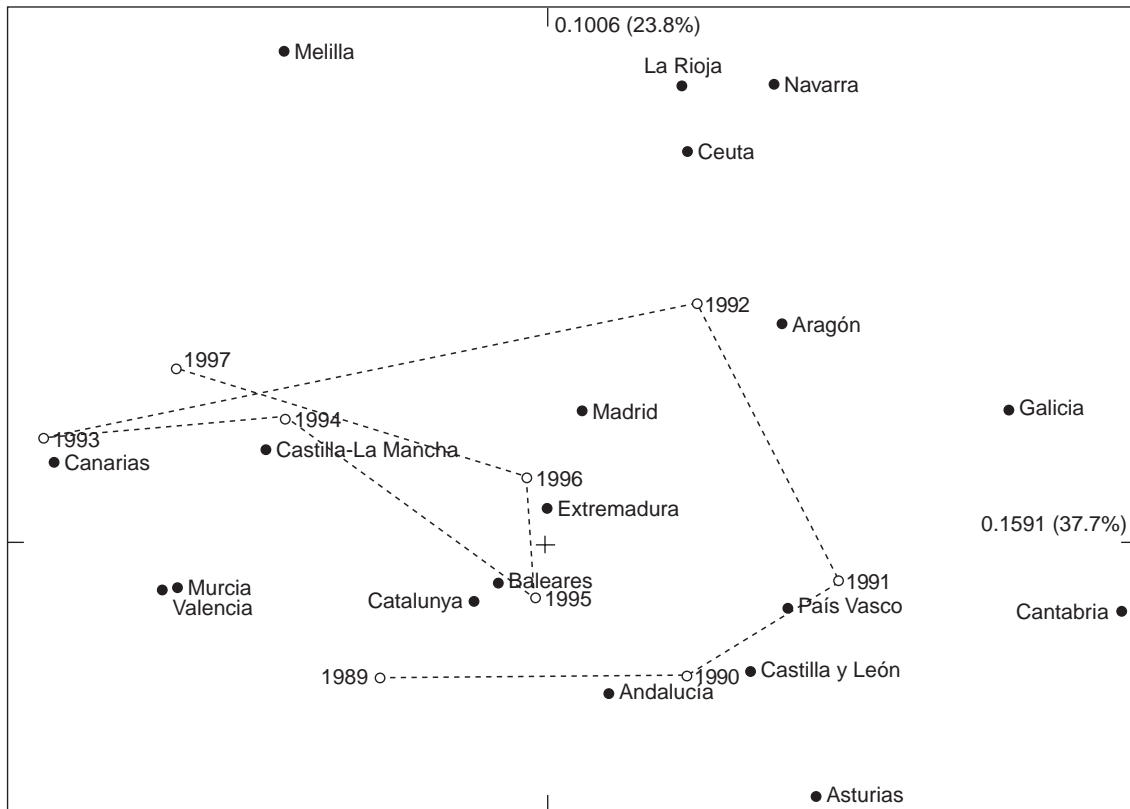
Figure 8. Correspondence analysis of measles trend data.
