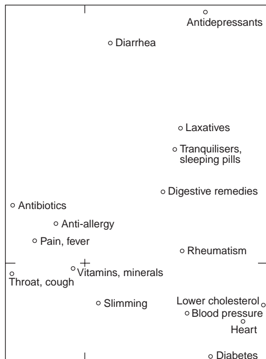
Figure 5. Multiple correspondence analysis, showing optimal scale values in two dimensions of «yes» responses to medicine types.
