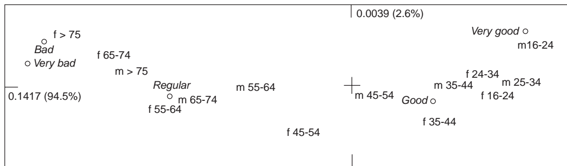
Figure 3. Correspondence analysis of table 3.
