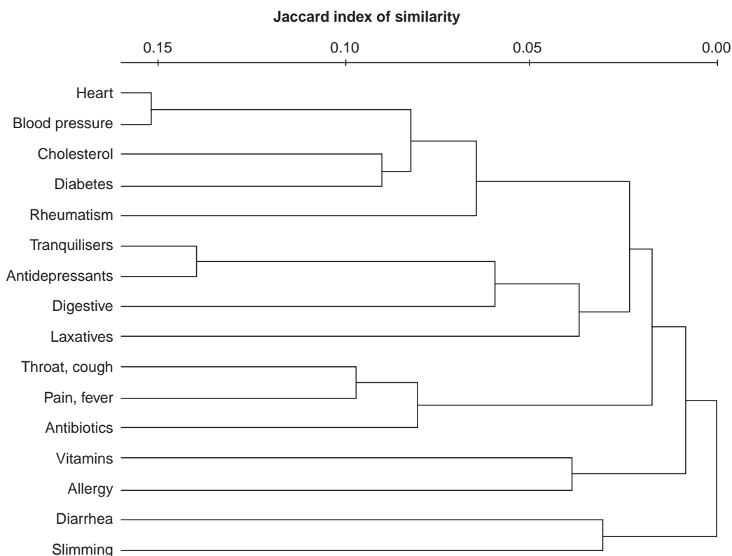
Figure 6. Hierarchical clustering tree of medicine types.
