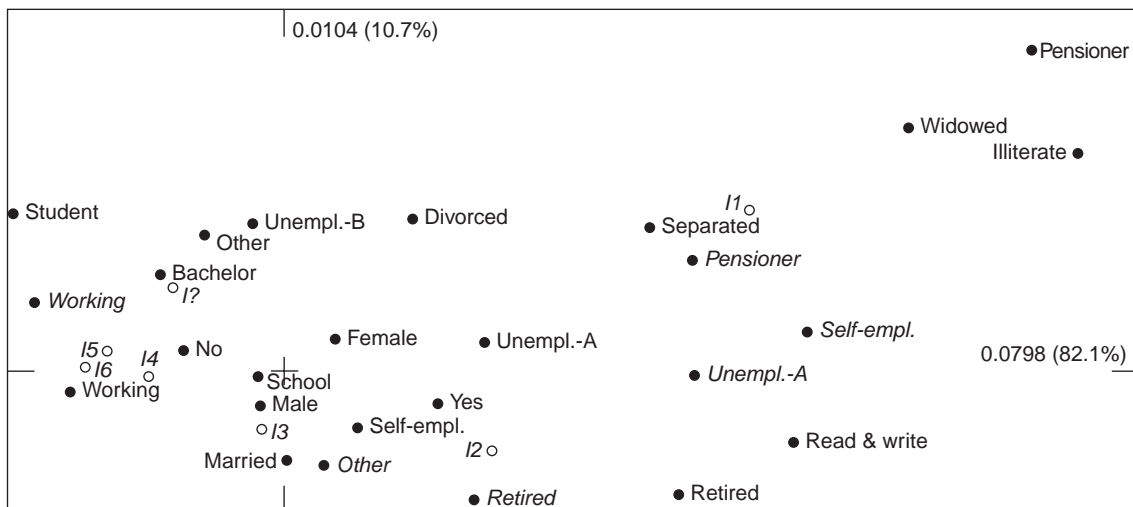
Figure 7. Correspondence analysis of table 6; the job status in italics refers to that of the head of the household (second part of table 6).
