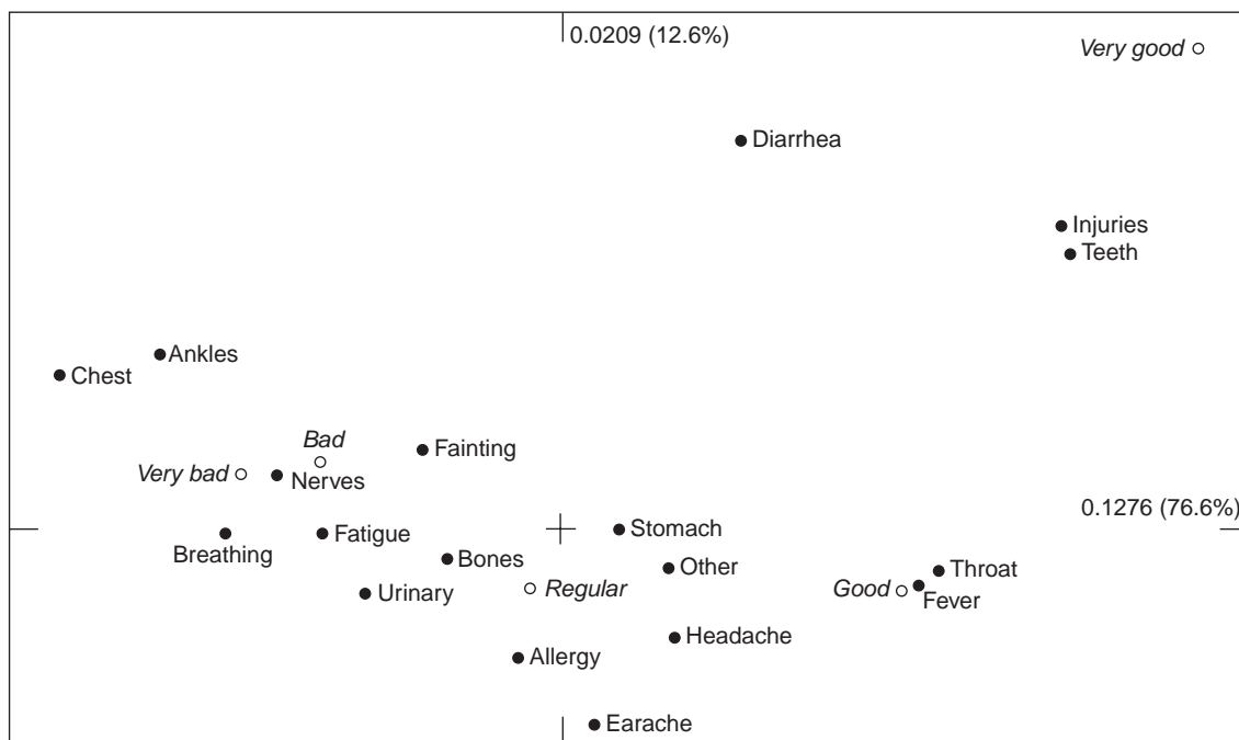
Figure 4. Correspondence analysis of table 4.
