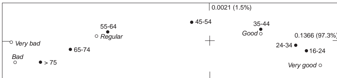
Figure 1. Correspondence analysis map of table 1.
