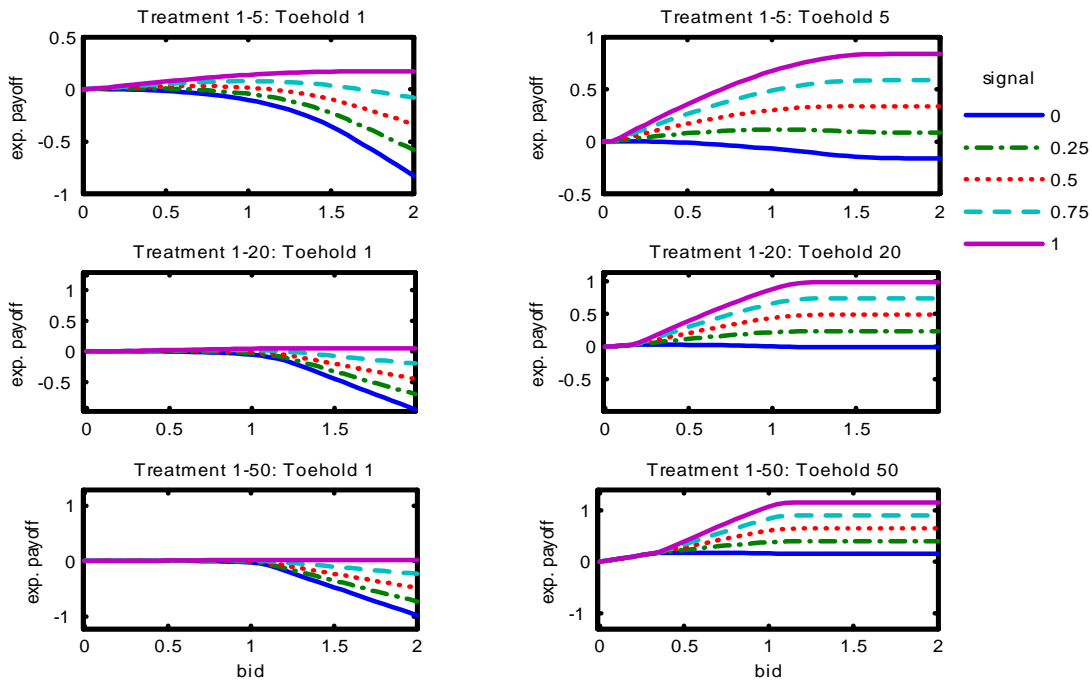
Figure 5: Payoff flatness in the various treatments. The various curves depict expected profits depending on bids (both scaled by 100) for signals 0, 25, 50, 75 and 100 given that the opponents play their equilibrium strategies.
