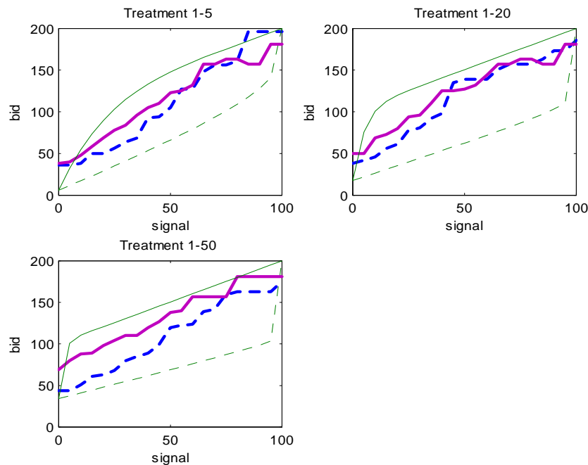
Figure 7: Best responses to actual bidding behaviour of the opponents. The dashed lines are the bids of the low type type, solid lines are bids of the high type. The thin lines depict the equilibrium best responses, while the thicker lines depict the best responses to the actual bid distributions.
