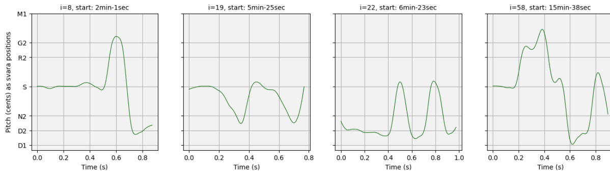
Figure 1: 4 pitch curves of the svara, ni
