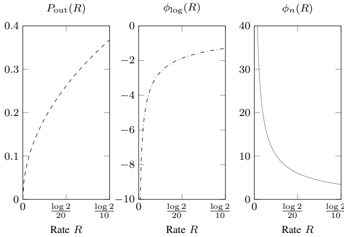
Fig. 1. Expansion terms P_{\text{out}}(R) , \phi_{\log}(R) and \phi_n(R) , for n = 10^5 .
