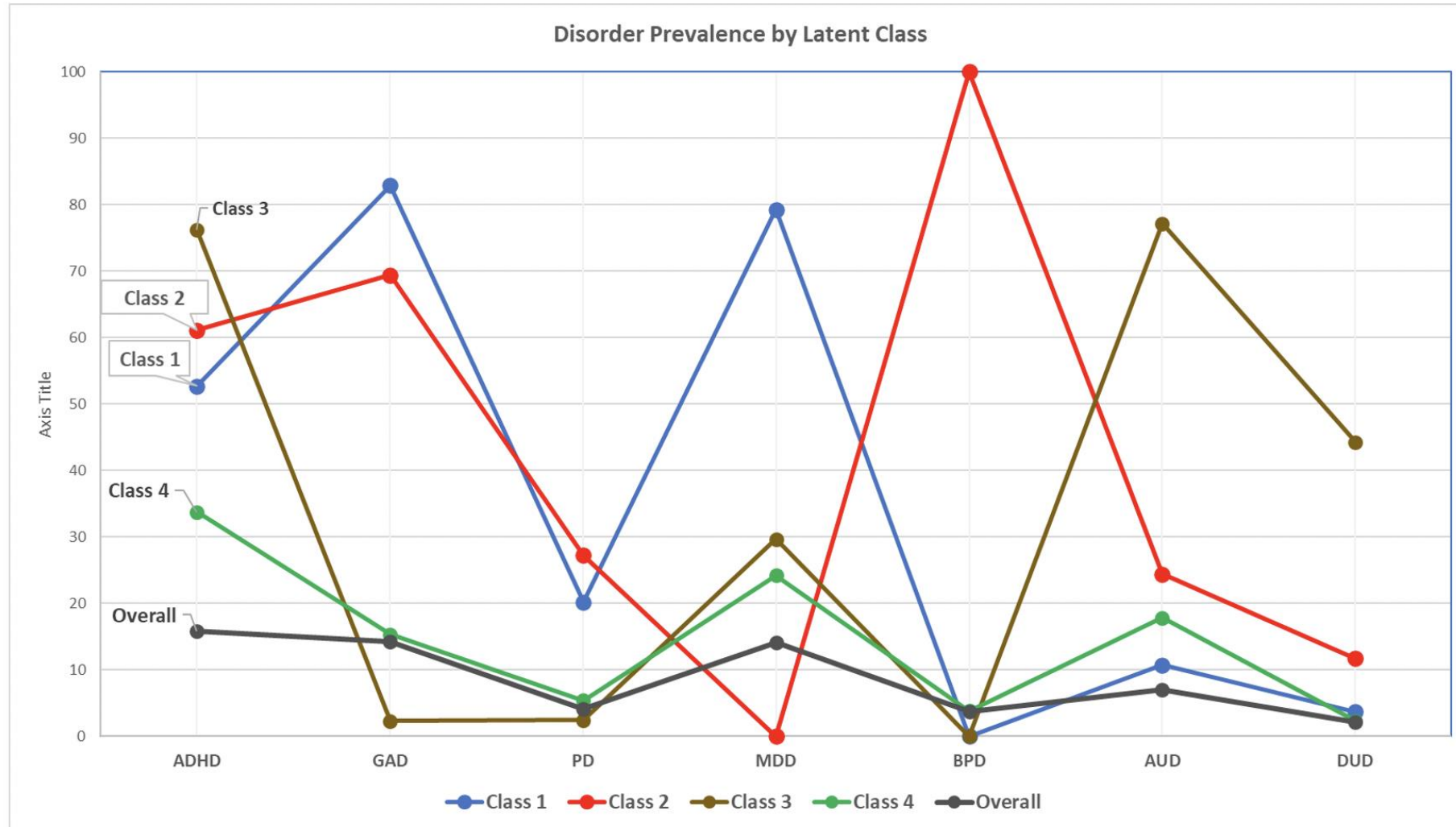
Figure 1. Prevalence of disorders within each latent class
