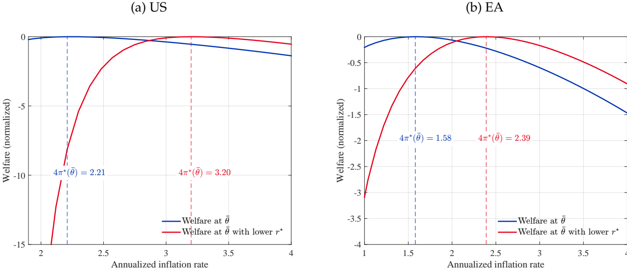
Figure C.1: \mathcal{W}(\pi, \mathbb{E}(\theta))
