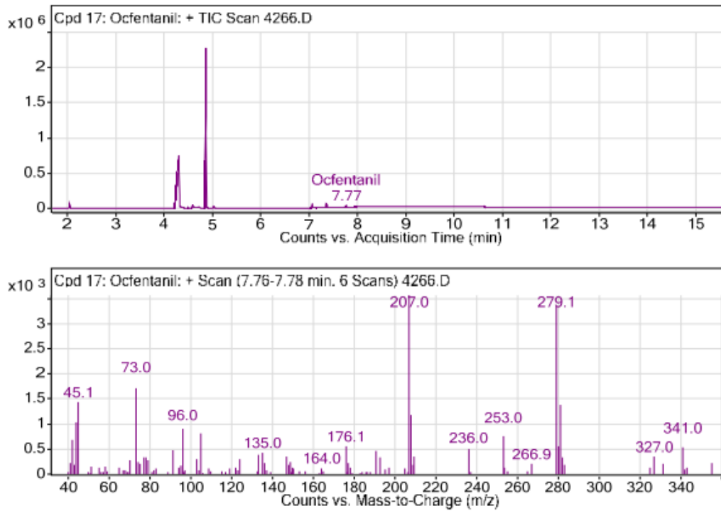
Figure 1: Results of GC/MS. Upper panel shows total ion chromatogram of sample #2 and lower panel shows mass spectra of ocfentanil.
