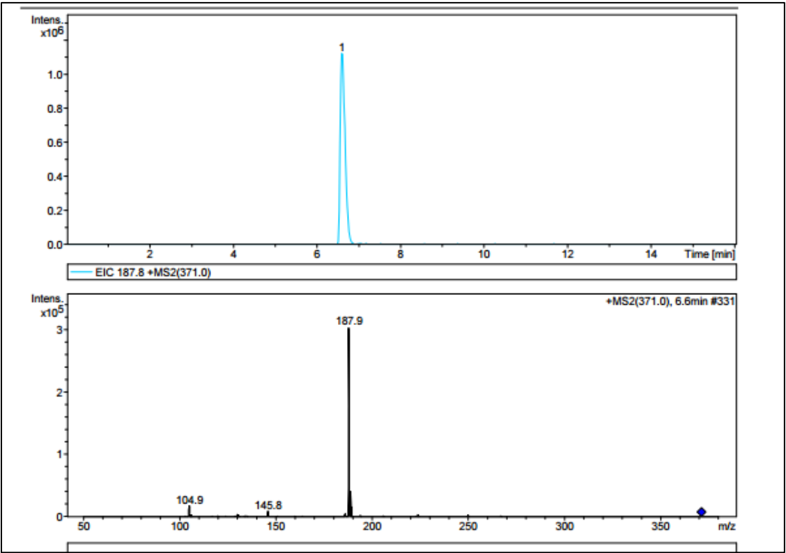
Figure 2: Results of ofentamil using LC/MS/MS with an ion trap in MRM mode
