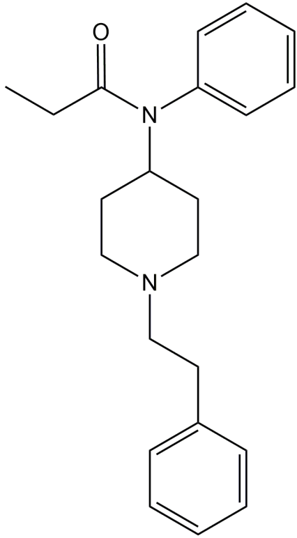
Fentanyl
