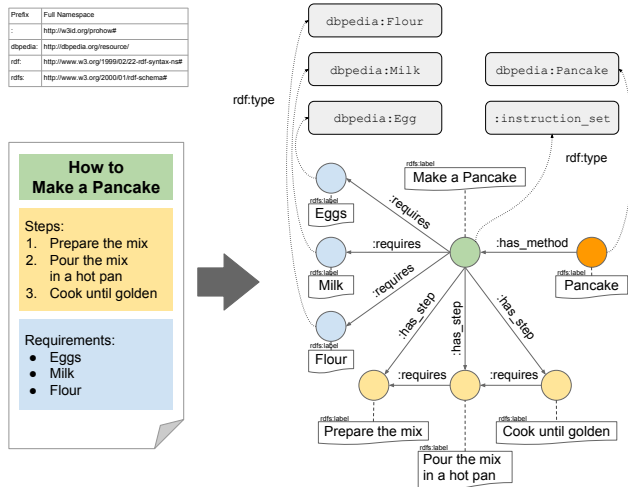
Figure 2: Example instantiation of PROHOW
