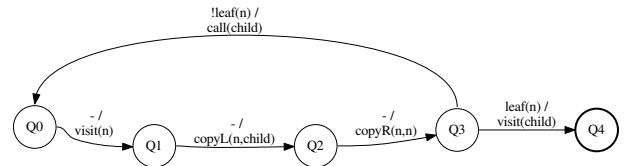
Figure 2: Hierarchical FSC C[n] that traverses a binary tree.
